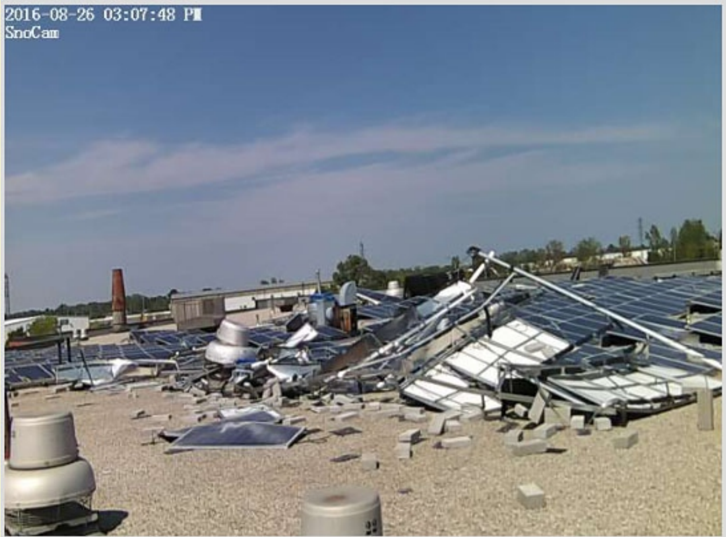
SolarVu SnoCam image of solar panel system damage after a tornado struck Windsor Ontario on Aug 24, 2016
